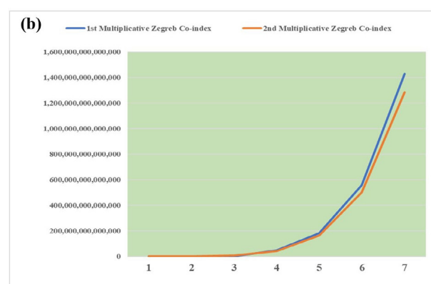
Figure 3: Comparison of first and second multiplicative Zagreb Co-indices
