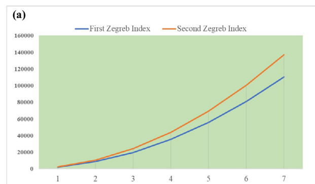
Figure 2: Comparison of first Zagreb index and second zagreb index
